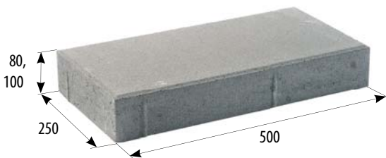
Layout dimensions
