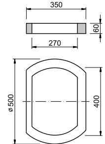
TBV-Q 10b/500×350/400×270/60 prsteneč
