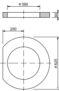
TBV-Q 10a/627/390/60 prsteneč
